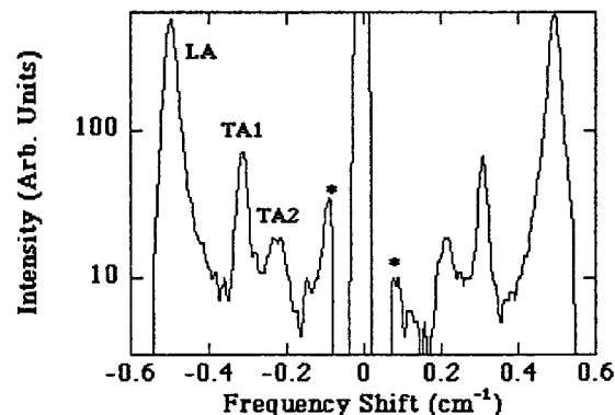
Figure 3. Typical Brillouin spectrum of polypropylene. LA and TA denote the longitudinal acoustic and transverse acoustic phonon, respectively. The features indicated by an asterisk are of instrumental origin.
