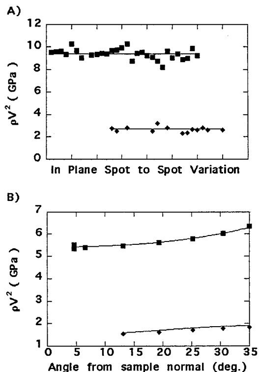
Figure 5. Elastic constants of PP-A0(X) measured in platelet (A) and backscattering (B) geometries. Solid squares and diamonds correspond to experimental longitudinal acoustic and transverse acoustic phonons, respectively. The lines represent the curve fits used to determine the C_{ij} in Table 1.
