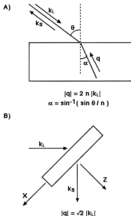
Figure 1. Scattering geometries used in Brillouin scattering experiments: (A) backscattering and (B) platelet. \mathbf{k}_L , \mathbf{k}_s , and \mathbf{q} are the incident, scattered, and phonon wave vectors, respectively, and k_L = 2\pi/\lambda_L , where \lambda_L is the wavelength of the laser radiation.
