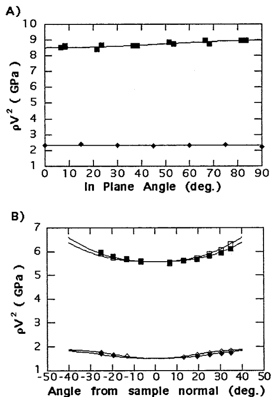
Figure 6. Elastic constants of PP-A1(11) measured in platelet (A) and backscattering (B) geometries. Squares and diamonds correspond to experimental longitudinal acoustic and transverse acoustic phonons, respectively; in (A) they correspond to values in the X - Y plane, in (B) the solid symbols are for the Z - Y plane and the open symbols are for the Z - X plane. The lines represent the curve fits used to determine the C_{ij} in Table 1.
