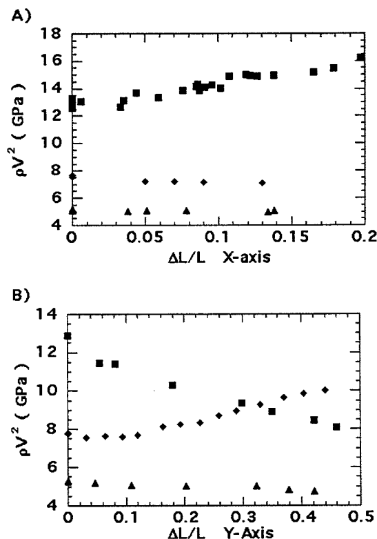
Figure 11. Variation in elastic constants ( C_{11} , squares; C_{22} , diamonds; C_{33} , triangles) with stretching of PP-BIAX film: along x -axis (A) and along y -axis (B).
