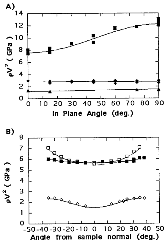
Figure 8. Elastic constants of PP-BIAX measured in platelet (A) and backscattering (B) geometries. Squares correspond to experimental longitudinal acoustic phonons. Diamonds and triangles correspond to experimental transverse acoustic phonons. In (A) they correspond to values in the X - Y plane. In (B) the solid symbols are for the Z - Y plane and the open symbols are for the Z - X plane. The lines represent the curve fits used to determine the C_{ij} in Table 1.
