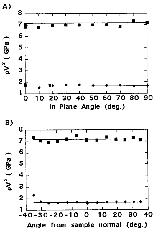
Figure 4. Elastic constants of PP-COMP measured in platelet (A) and backscattering (B) geometries. Solid squares and diamonds correspond to experimental longitudinal acoustic and transverse acoustic phonons, respectively. The lines represent the curve fits used to determine the C_{ij} in Table 1.
